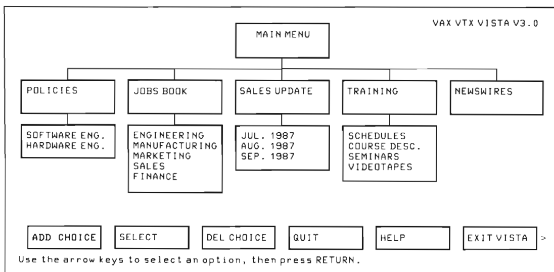
Figure 4 Sample VISTA Menu Structure
