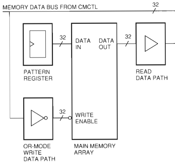
Figure 2 OR-mode Circuit
