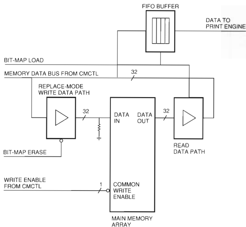
Figure 3 Scan-erase Circuit
