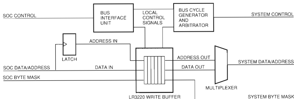
Figure 5 Write Buffer
