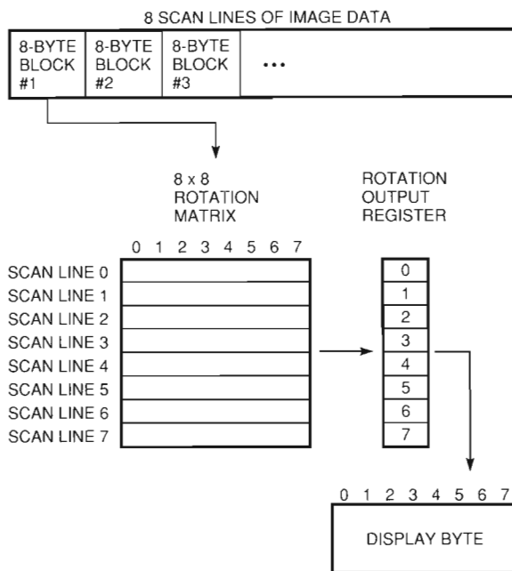
Figure 5 Rotation Matrix
