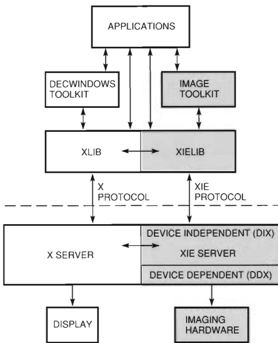
Figure 7 X/XIE Architecture
