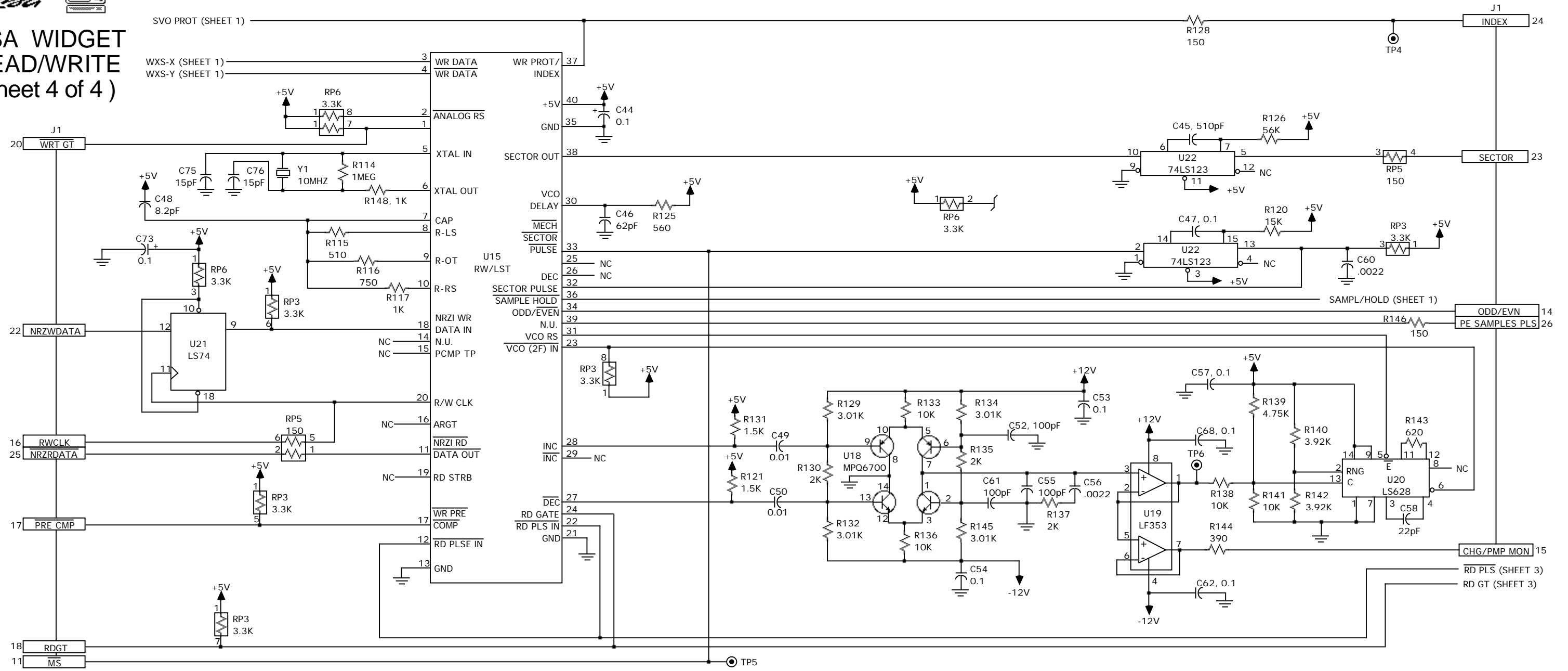
Lisa Widget Read/Write Circuit Sheet 4 of 4
