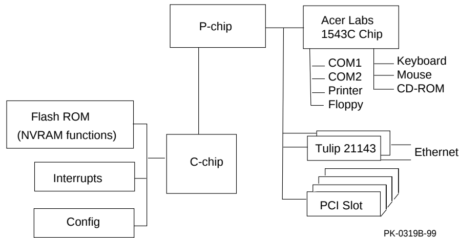
Block Diagram of I/O Control
